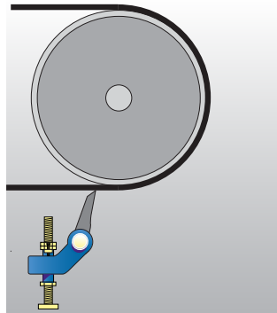
Primary Scraper Position
