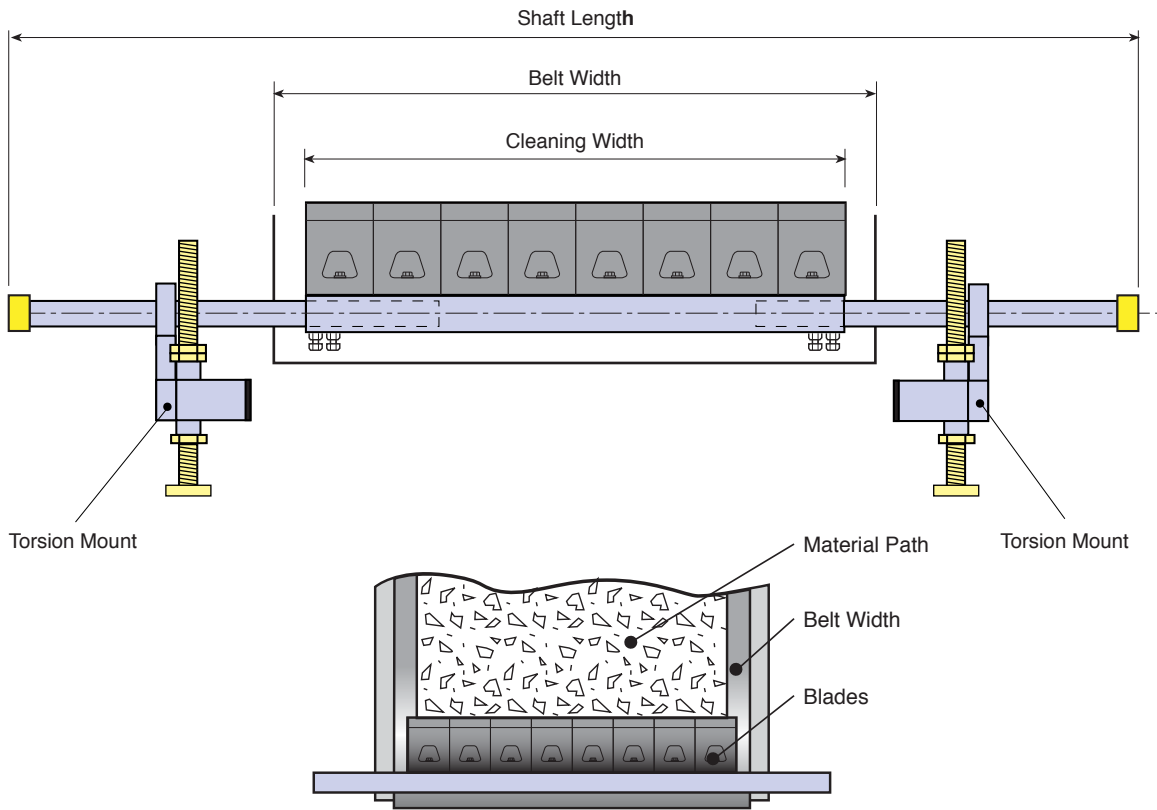
Blade to match belt width
