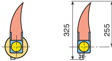
Scraper Blade Assembly
