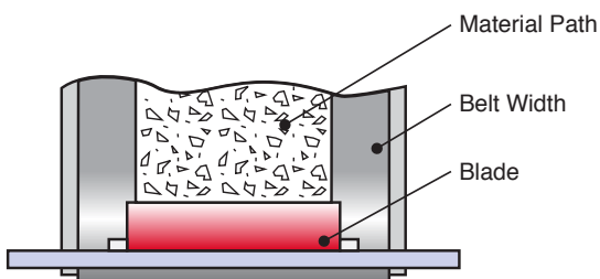
Blade to match material width - 'D'
