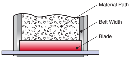
Blade to match belt width - 'C'
